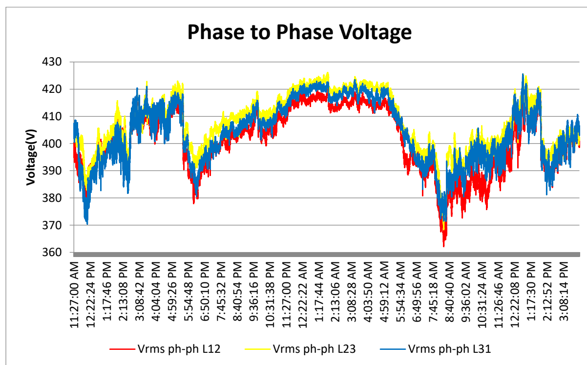
Graph 4: Voltage trend
